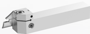
Square shank integral face grooving holders*
